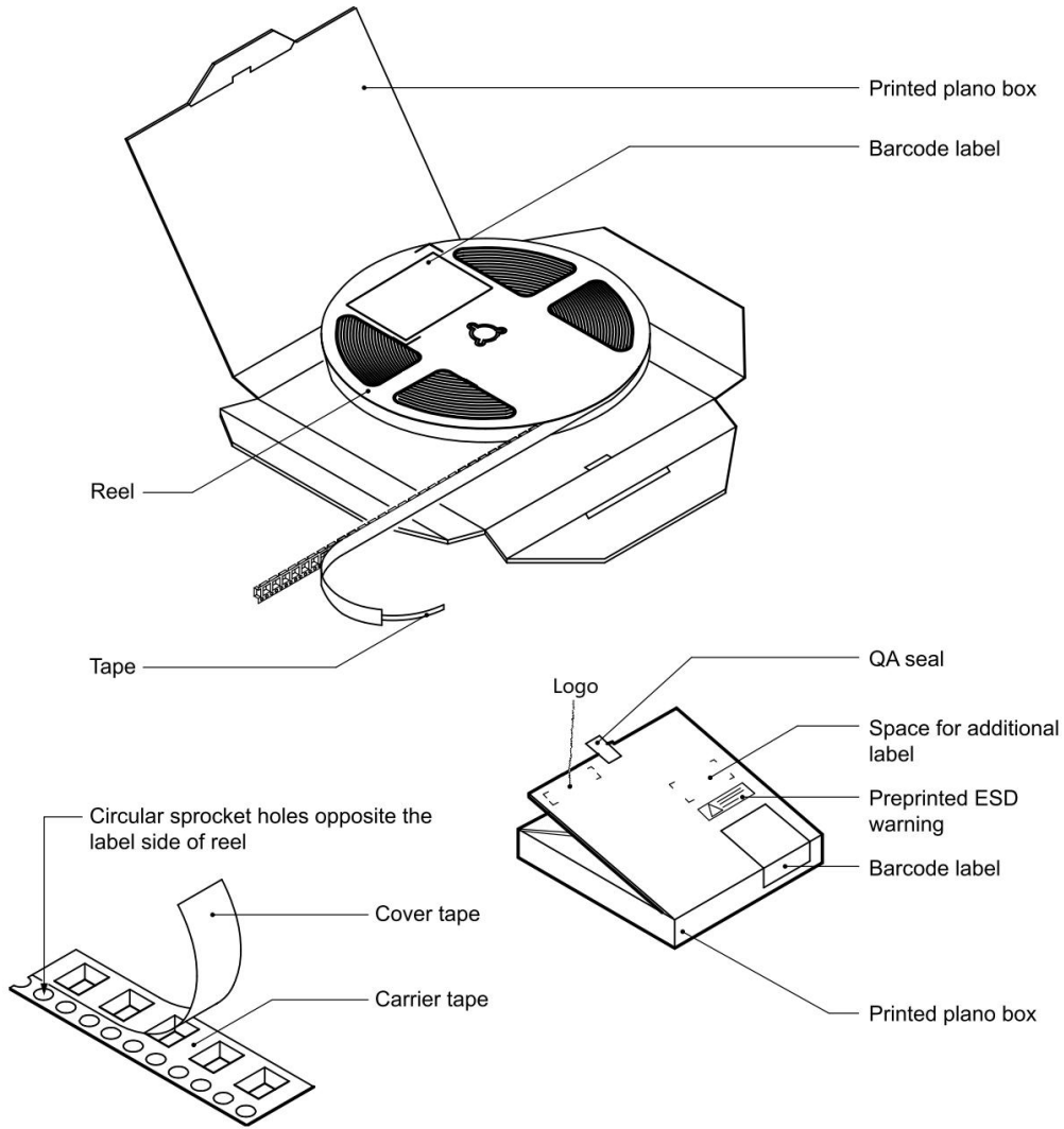
Figure1. Reel pack for SMD
